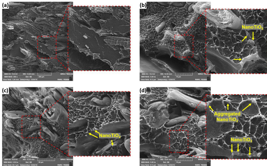
FIGURE 4 FESEM micrographs of the WPC filled with TiO 2 nanoparticles. (a) 0%, (b) 1%, (c) 3%, (d) 5%.
