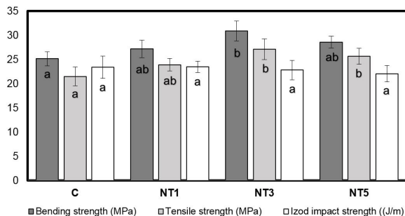
FIGURE 1 Mechanical strengths of samples: (C) Control, (NT1) 1% Nano TiO 2 , (NT3) 3% Nano TiO 2 , (NT5) 5% Nano TiO 2 .
