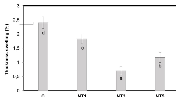
FIGURE 3 Thickness swelling of samples: (C) Control, (NT1) 1%Nano TiO 2 , (NT3) 3%Nano TiO 2 , (NT5) 5%Nano TiO 2 .
