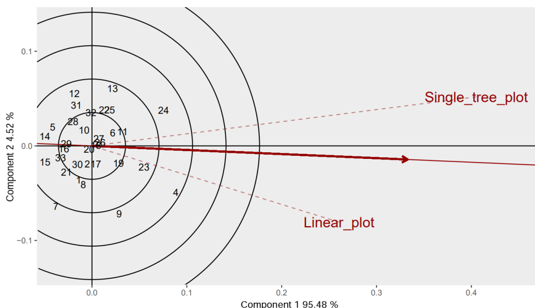
FIGURE 1 GGE Biplot “Discriminant Power vs. Representativeness” generated with BLUP values from the individual volume of Eucalyptus spp. clones in the linear plot and single-tree plot designs at five years of age. The clones were established at the study site in Lençóis Paulista, São Paulo State.
